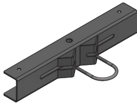
Floodlighting bracket Art.Nr. 920-9xx
